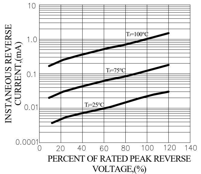
FIG.4-MAXIMUN REVERSE CHARACTERISTICS
