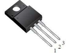
TO-220F-3L MBR20100FCT
